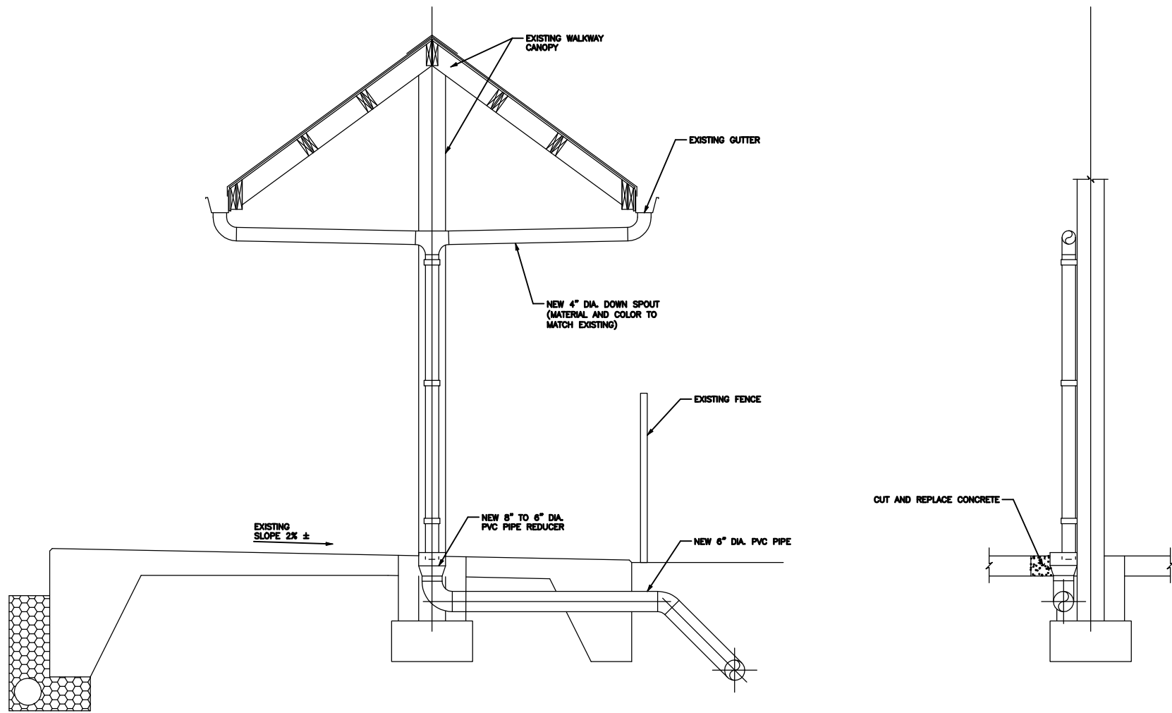
DETAIL - NEW DOWN SPOUT AND ROOF DRAIN N.T.S.
